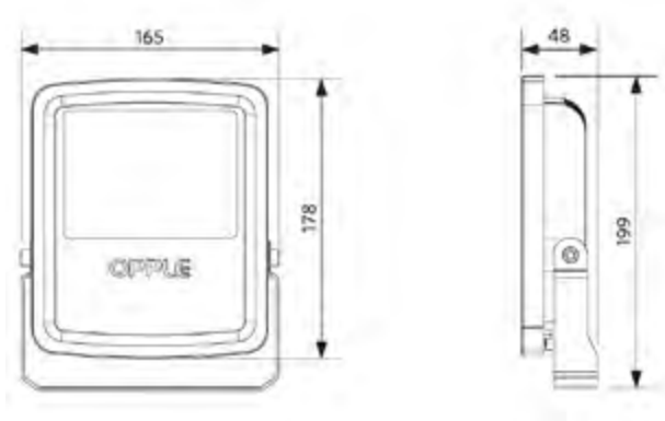
LEDflood-E2 Re283
