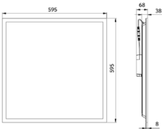
LEDPanelS-E4 Re295-32W
