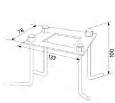
LEDBollard-Luke-E Concrete-Mounting-Kit
