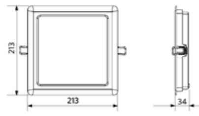
LEDDownlightRc-SI-E Sq200
