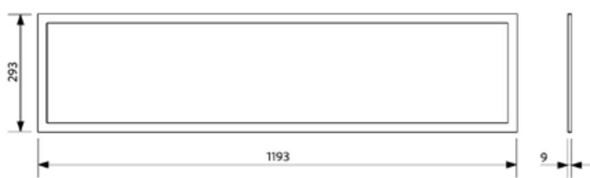
LEDPanelRc-S-E2 Re295
