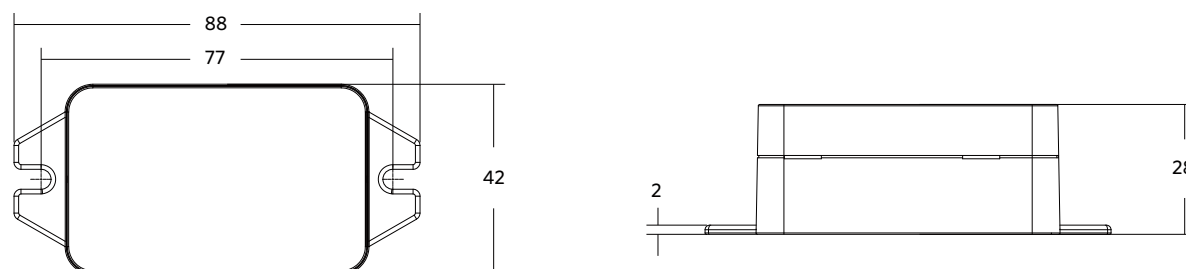
821017001400 - LEDSmart-BLE-10V-Converter
