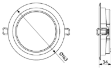
LEDDownlightRc-SI-E Rd150
