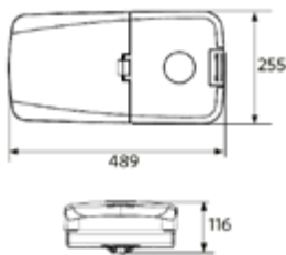
Pole Adapter-Road-St-P2-60mm
