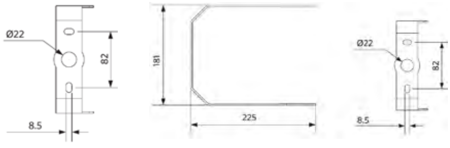
LEDHighbay-P4 Bracket-D420
