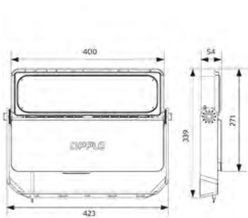
LEDfloodMo-P Re570
