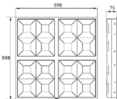
LEDPanelRc-G Sq598
