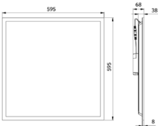
LEDPanelS-B3 Re295-32W
