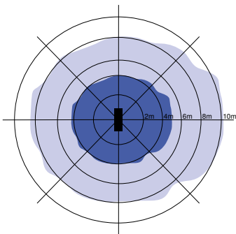
Installation - Low ceiling Suggested installation height 9m
