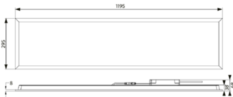
LEDPanelS-B3 Re295-32W
