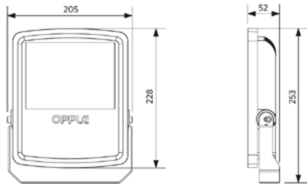
LEDflood-E Sensor
