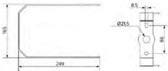
LEDHighbay-E2 Bracket-L249
