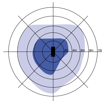
Installation - High ceiling Suggested installation height 15m
