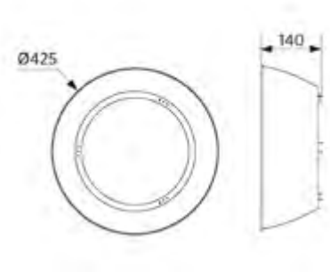
LEDHighbay-P4 Reflector-D420
