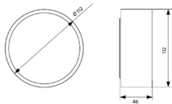
LEDCeilingLu-E Rd112
