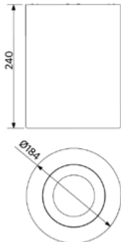
LEDDownlightRc-P-R150-Surface-Module
