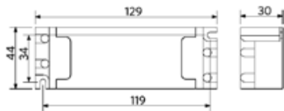
LEDPanelRc-S-E2 Driver
