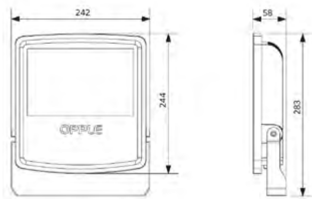
LEDflood-E2 Re283
