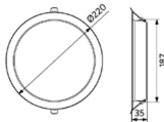
LEDDownlightCo-E Rd200
