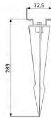
LEDSpotProjector-E Spike
