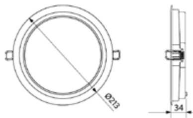
LEDDownlightRc-SI-E Rd200
