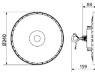
LEDHighbay-E2 Reflector-Rd507
