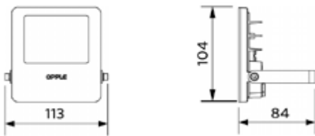
LEDflood-E Sensor
