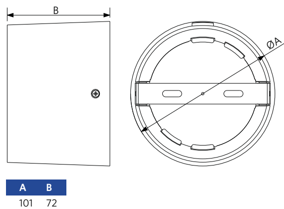
560098000600 - LEDSmart-Sensor Surface-Module-WH
