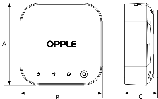
821011002600 - LEDSmart-BLE2-DALI-Connect-Box
