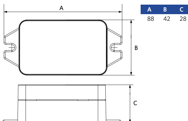
821017003600 - LEDsmart-BLE2-Relay-250W-DIM
