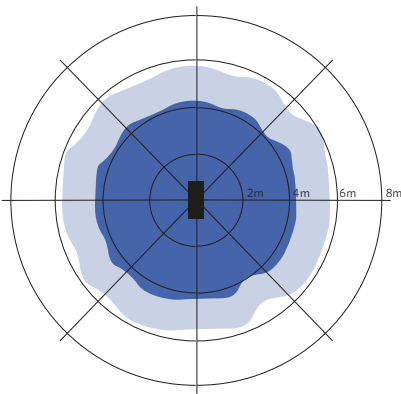
Installation - Ceiling mounted Suggested installation height 2.5-6m
