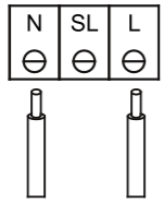
2. Non-Maintained
