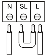
1. Maintained
