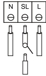
3. Switched Maintained
