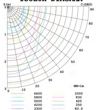
ISOLUX DIAGRAM
