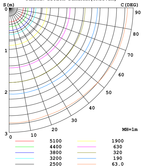
PLANAR ISOLUX DIAGRAM (UNIT: lx)
