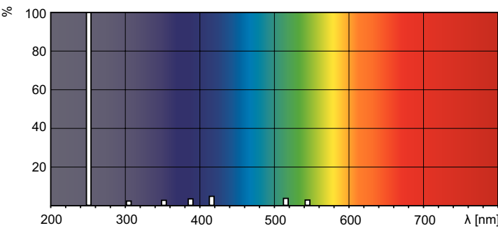
Spectral Power Distribution Colour - TUV 30W 1SL/25-Latest
